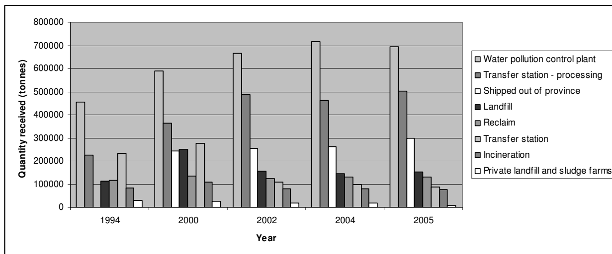
Figure F: Quantities of hazardous and liquid industrial waste transfers received in Ontario by receiving facility type, 1994 – 2005
